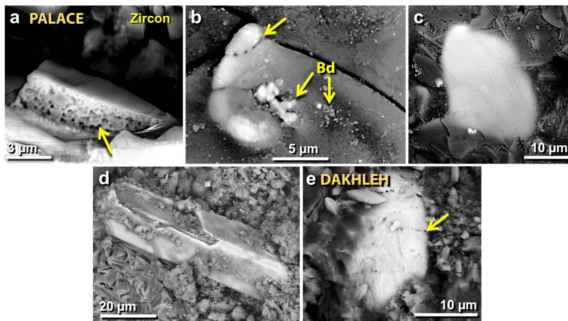
Figure 30. SEM images of melted zircon grains. (a) Melted TeH zircon grain with bubbles at yellow arrow due to high-temperature dissociation and/or entrapped porosity. (b) Melted TeH zircon grain decorated with bubbles along the fracture line at upper arrow; arrows labeled “Bd” point to bright granular baddeleyite, ZrO_2 , formed during the high-temperature dissociation of zircon. (c) Almost fully melted TeH zircon grain mixing into the Ca–Al–Si matrix. (d) A typical unmelted zircon grain from TeH with straight, euhedral edges. Grain shows cracks on the top surface from possible thermal or mechanical damage. (e) For comparison, from cosmic airburst/impact at Dakhleh Oasis in Egypt: melted zircon decorated with lines of bubbles (arrow).
