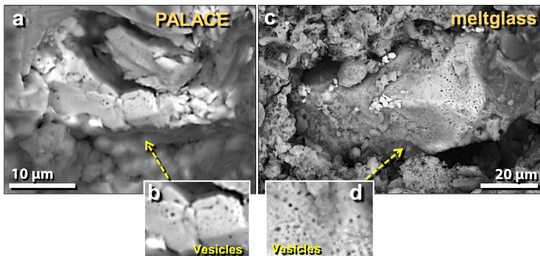
Figure 39. SEM images of melted iron and titanomagnetite in mudbrick meltglass from the palace. (a) Shattered elemental Fe grain containing < 0.1\text{ wt.}\% oxygen as determined by SEM-EDS; (b) close-up showing surface porosity. (c) Titanomagnetite grain showing surface porosity; (d) close-up showing aligned porosity possibly along former grain boundaries. The cause of the porosity is uncertain, but because these grains are associated with other high-temperature melted minerals, we propose that this porosity resulted from exposure to high temperatures.
