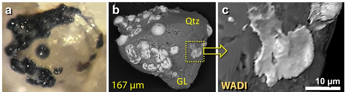
Figure 28. Fe-rich spherules embedded in meltglass. (a) Optical photomicrograph of a 167- \mu\text{m} -wide piece of meltglass with embedded Fe-rich spherules. (b) SEM image of same grain as in panel ‘a’. Melted quartz grain (Qtz) is embedded in Ca–Al–Si-rich matrix, which has the same composition as melted mudbrick. (c) SEM close-up image of the boxed area and panel ‘b’, showing splattered Fe-rich spherule.
